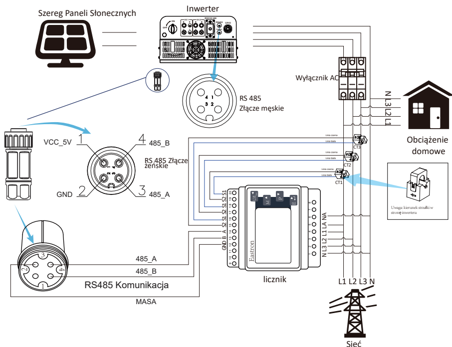
Pic 7.14 Connection diagram of Eastron meter
